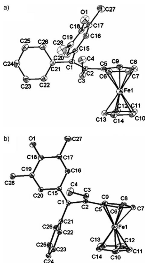
Figure 1. ORTEP views of a) (Z)- 4 and b) (E)- 4a with thermal ellipsoids presented at 50% probability. Selected bond lengths [Å] for 4 : C18–O1 1.402(4), C15–C16 1.401(4), C16–C17 1.399(4), C17–C18 1.407(5), C15–C1 1.510(4), C1–C2 1.361(4), C2–C3 1.536(4); for 4a : C18–O1 1.246(3), C15–C16 1.459(4), C16–C17 1.361(4), C17–C18 1.481(4), C15–C1 1.381(4), C1–C2 1.512(4), C2–C3 1.343(4).
