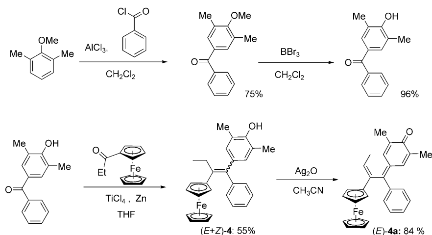
Scheme 1. Synthesis of 4 and 4a .
